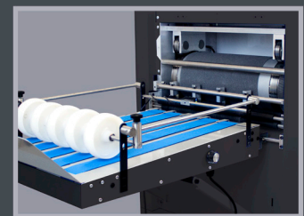
Conveyor System with Scrap Separator
